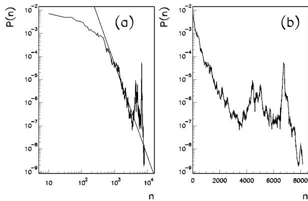
FIG. 4. Quantum stationary distribution for k = 50 , and T = 0.01 . The map has been iterated 10^6 times. The final distribution is obtained by averaging over the last 10^5 kicks. The initial state is \psi_n = \delta_{n,0} . (a) Log-log scale. The line n^{-4} has been drawn to guide the eye. (b) Log scale.
