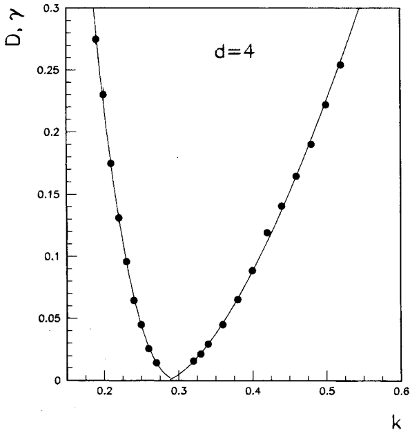
Fig. 5. Inverse localization length (left side) and diffusion rate (right side) for d = 4 . Lines are the separate fits: \gamma = \gamma_0(k_{cr} - k)^v with \gamma_0 = 66 (10), k_{cr} = 0.306 (2) and v = 2.53 (1) with \chi^2 = 10.2 and D = D_0(k - k_{cr})^s with D_0 = 2.29 (2), k_{cr} = 0.283 (3) and s = 1.52 (5) with \chi^2 = 111 . A similar fit for \gamma_i = \gamma_{0i}(k_{cr} - k)^{v_i} gives \gamma_{0i} = 85 (28), k_{cr} = 0.305 (5), v_i = 2.59 (2) and \chi^2 = 4.5 . Here 10–100 random configurations have been iterated up to 10^7 kicks. Data errors are within the symbol size.
