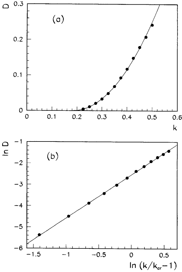
Fig. 10. d = 5 . (a) Diffusion rate vs. k , three parameters fit (full line) gives: D = 2.56 (6) (k - 0.180) (2) 2.04 (3) with \chi^2 = 36.1 ; (b) logarithm of diffusion rate vs. \ln(k/k_{cr} - 1) where k_{cr} is extracted from (a). Best fit (full line) has the slope s = 2.039 (9).
