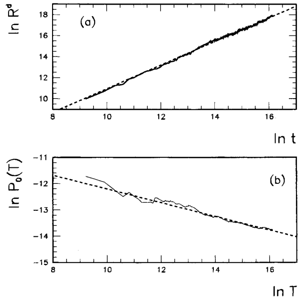
Fig. 8. The same as Fig. 7 but for d = 4 near the critical point at k = 0.27 . Results from fit gives R^d \sim t^{1.12(3)} and P_0(T) \sim T^{-0.26(3)} .
