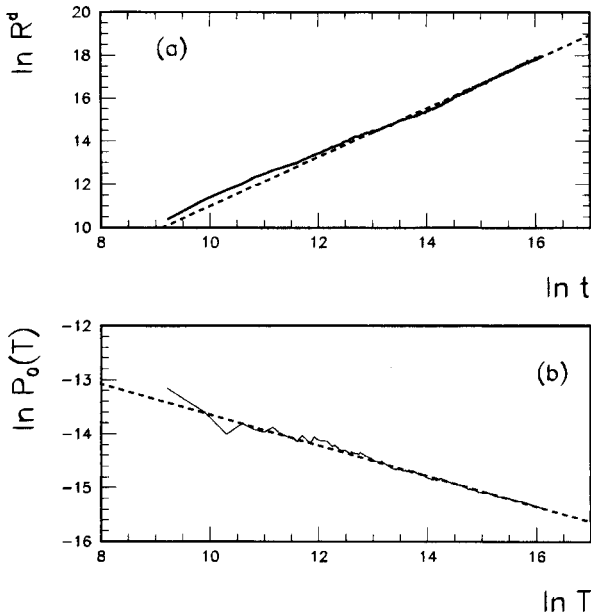
Fig. 7. d = 3 . Study near the critical point at k = 0.48 . (a) Behavior of R^d = \sum_n |n|^d |\psi_n|^2 in time. Best fit (dashed line) gives R^d \sim t^{1.13(3)} . (b) Behavior of the logarithm of the integrated probability to stay P_0(T) as a function of the logarithm of time T . Here is P_0(T) = (1/T) \int_0^T dt |\psi_{n_0}(t)|^2 and the initial state vector is \psi(t=0) = \delta_{n,n_0} . Best fit (dashed line) gives P_0(T) \sim T^{-0.28(3)} . One random configuration has been considered. Basis is N = 4096 .
