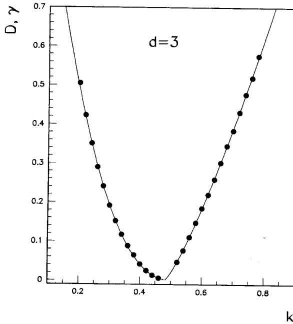
Fig. 3. Inverse localization length (left side) and diffusion rate (right side) for d = 3 . Lines are the separate fits: \gamma = \gamma_0(k_{cr} - k)^\nu with \gamma_0 = 8.01 (1), k_{cr} = 0.509 (1) and \nu = 2.37 (1) with \chi^2 = 10.5 and D = D_0(k - k_{cr})^s with D_0 = 2.56 (2), k_{cr} = 0.479 (1) and s = 1.25 (1) with \chi^2 = 32.6 . A similar fit for \gamma_i = \gamma_{0i}(k_{cr} - k)^{\nu_i} gives \gamma_{0i} = 3.7 (3), k_{cr} = 0.489 (4), \nu_i = 1.71 (6) and \chi^2 = 15.4 . Here 10–100 random configurations have been iterated up to 10^7 kicks. Data errors are within the symbol size.
