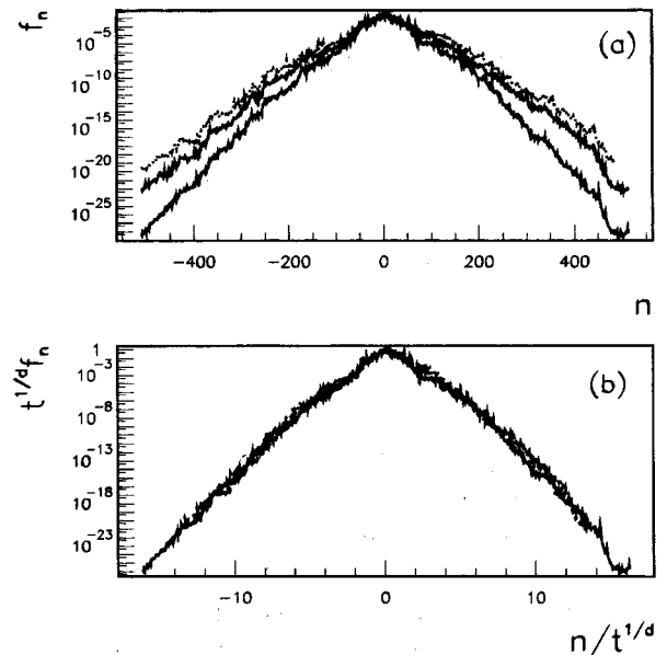
Fig. 9. Rescaling of the distribution function in the critical region ( k = 0.27 ) for d = 4 . (a) The averaged (over 10^4 kicks) probability distribution over the unperturbed basis f_n taken at three different times t_1, 2t_1, 3t_1 where t_1 = 10^6 , shows that as the time goes on the distribution increases its size. (b) The same as (a) but in the rescaled variables t^{1/d} f_n and n/t^{1/d} (since at the critical point |n|^d \sim t with d = 4 ).
