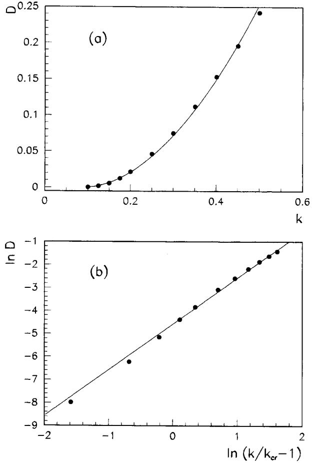
Fig. 11. d = 11 . (a) Diffusion rate vs. k , three parameters fit gives: D = 1.35 (1) (k - 0.0924) (5) 1.87 (1) with \chi^2 = 310 ; (b) logarithm of diffusion rate vs. \ln(k/k_{cr} - 1) where k_{cr} is extracted from (a). Best fit (full line) has the slope s = 1.99 (5).
