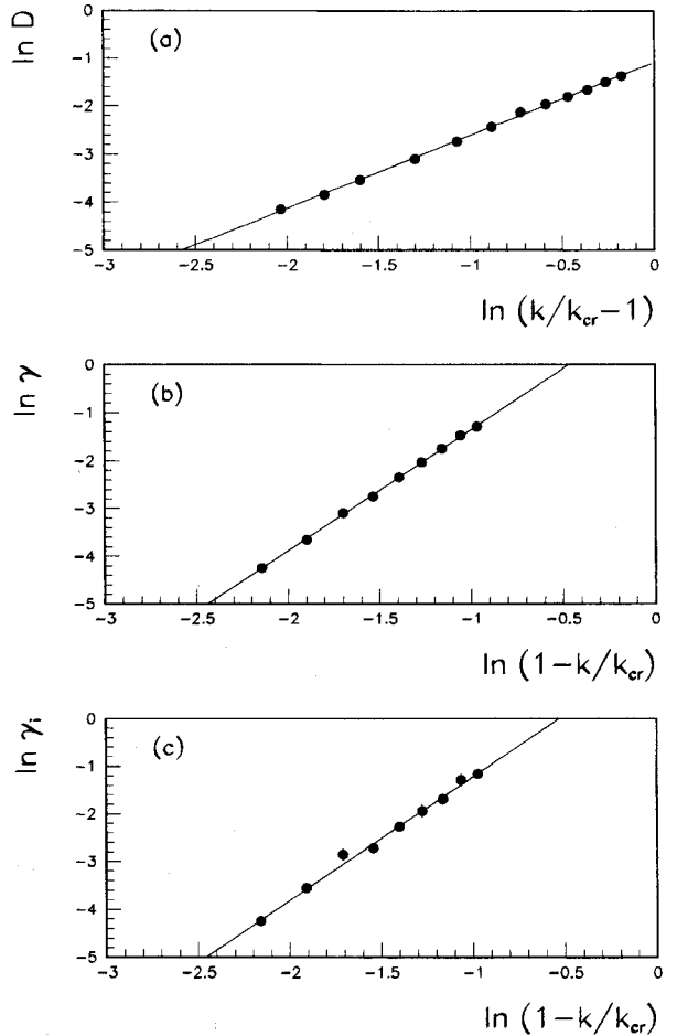
Fig. 6. d = 4 . (a) Logarithm of diffusion rate vs. \ln(k/k_{cr} - 1) where k_{cr} is extracted from the separate fit (Fig. 5). Straight line is the best fit line with slope s = 1.519 (4) and \chi^2 = 115 . (b) Logarithm of the inverse localization length vs. \ln(1 - k/k_{cr}) where k_{cr} is extracted from the separate fit (Fig. 5). Straight line is the best fit line with slope v = 2.534 (5) and \chi^2 = 91.81 . (c) Logarithm of the participation ratio \gamma_i vs. \ln(1 - k/k_{cr}) where k_{cr} = 0.305 (5) is extracted in a similar way from a three parameter fit. Here the straight line has slope v_i = 2.59 (2) and \chi^2 = 4.5 . Here 10–100 random configurations have been iterated up to 10^7 kicks. Errors are within the symbol size.
