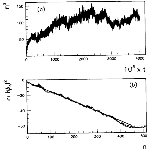
Fig. 2. (a) Behavior of the second moment on time for k = 0.24 , d = 4 (localized side). Basis is N = 1024 . (b) Logarithm of the averaged distribution function between t = 0.3995 \times 10^7 and t = 0.4 \cdot 10^7 . On x -axis we put n . Line represents the fitted localized distribution with l = 15.4 .
