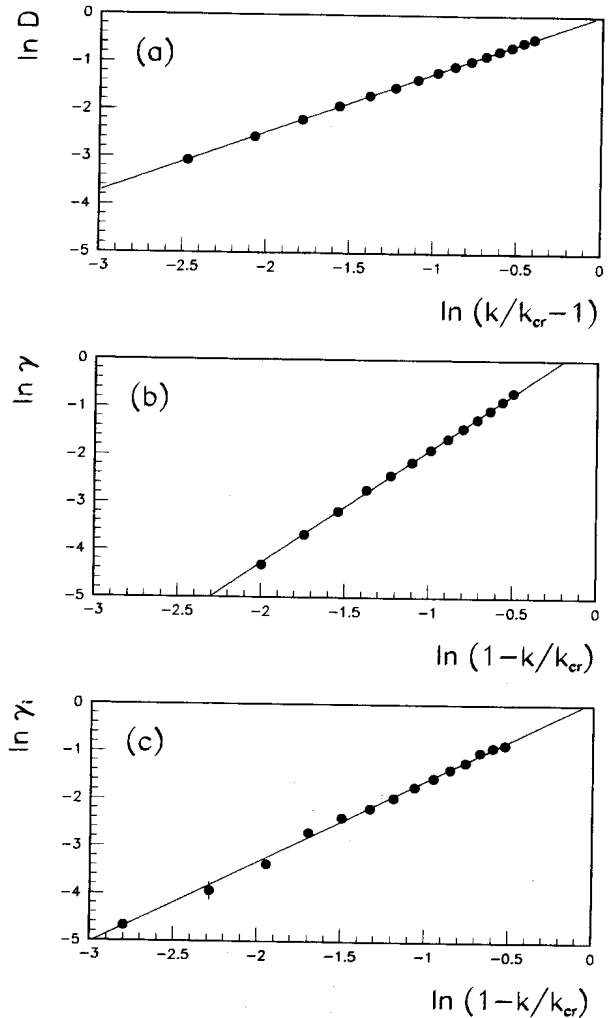
Fig. 4. d = 3 . (a) Logarithm of diffusion rate vs. \ln(k/k_{cr} - 1) where k_{cr} is extracted from the separate fit (Fig. 3). Straight line is the best fit line with slope s = 1.248 (5) and \chi^2 = 10.6 . (b) Logarithm of the inverse localization length vs. \ln(1 - k/k_{cr}) where k_{cr} is extracted from the separate fit (Fig. 3). Straight line is the best fit line with slope \nu = 2.374 (9) and \chi^2 = 33.8 . (c) Logarithm of the participation ratio \gamma_i vs. \ln(1 - k/k_{cr}) where k_{cr} = 0.489 (4) is extracted in a similar way from a three parameter fit. Here the straight line has slope \nu_i = 1.71 (6) and \chi^2 = 16.3 . Here 10–100 random configurations have been iterated up to 10^7 kicks. Errors are within the symbol size.
