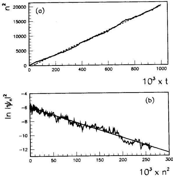
Fig. 1. (a) Behavior of the second moment on time for k = 0.33 , d = 4 (diffusive side). Dashed line is the fitted diffusion coefficient D = 0.0205 . Fourier basis is N = 1024 . (b) Logarithm of the averaged distribution function between t = 0.995 \times 10^6 and t = 10^6 ( t = number of kicks). Full line is the best fit gaussian which gives a diffusion coefficient D = 0.0229 . On x -axis we put n^2 .
