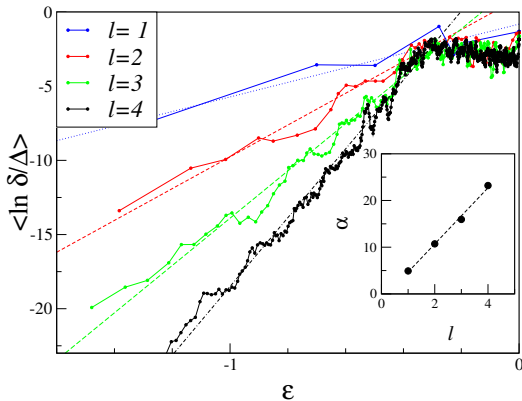
FIG. 3: (Color online) Average (over energy bins) of \langle \ln(\delta/D) \rangle vs the specific energy \epsilon , for N = 6 , \eta = 1 and different l , as indicated in the legend. Here D is the average level spacing. Also shown (dashed and dotted style) the linear fit. Inset: the linear dependence of the slopes \alpha with l . Linear fitting is \alpha = -1.3 + 6l .
