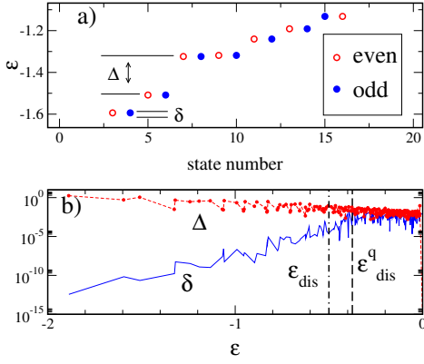
FIG. 1: (Color online) N = 6 l = 3 \eta = 1 . a) Doublet structure of the low energy region of the spectrum. The different parity of the states constituting the doublets is shown. We also indicated the level distance among even eigenstates, \Delta . b) the splitting of the doublets, \delta , vs the specific energy, \epsilon = E/N (blue line) and the nearest neighbor level spacing \Delta(\epsilon) (red line). Also shown as vertical lines: the quantum disconnection border, \epsilon_{dis}^q (dashed), computed analytically from Eq.(2), and \epsilon_{dis} (dashed-dotted).
