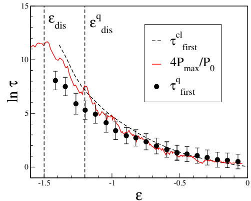
FIG. 4: (Color online) The quantum average reversal time, \tau (circles), as a function of \epsilon is shown for the case N = 6 , \eta = 1 and l = 4 , are compared with the classical ones (dashed black line), showing a good agreement above \epsilon_{dis}^q and a deviation near \epsilon_{dis} . Also shown, as a full line 4P_{max}/P_0 averaged over close eigenfunctions.
