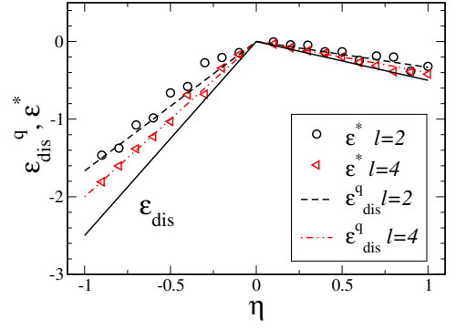
FIG. 2: (Color online) \epsilon_{dis}^q (dashed lines) and \epsilon^* (symbols) for different l values vs \eta . Data are N = 6 , l = 2, 4 . Also shown (as full line) \epsilon_{dis} that showing, at the same time, the agreement between \epsilon_{dis}^q and \epsilon^* and their common semiclassical limit \epsilon_{dis} .
