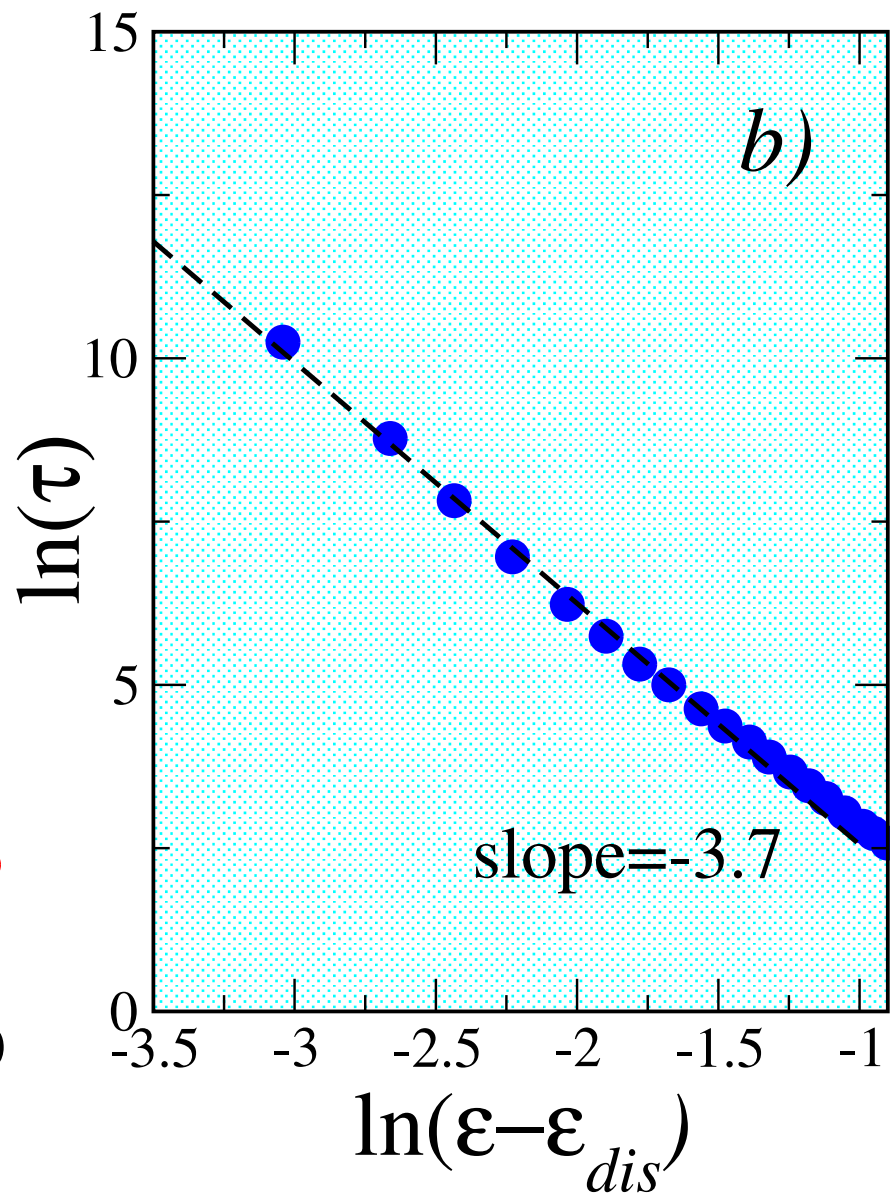
1D chain \alpha=2
