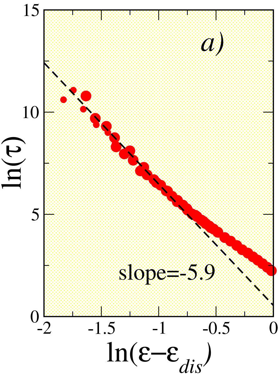
3D cube \alpha=\infty
