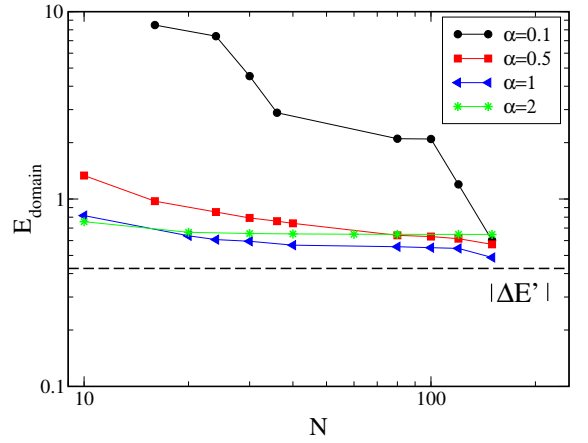
FIG. 5: (Color online) Domain wall energy as a function of N for different \alpha values, as indicated in the legend, and \eta = 0.9 . Also shown as horizontal dashed line |\Delta E'| = \eta^2/(1 + \eta) .
