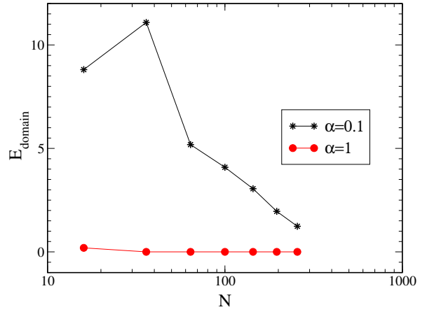
FIG. 9: (Color online) Domain energy as a function of the number of lattice spins, for the 2-d square lattice and \eta = 0.5 , asterisks ( \alpha = 0.1 ), circles ( \alpha = 1 ). For \alpha > 1 , E_{domain} becomes smaller than the computer precision.
