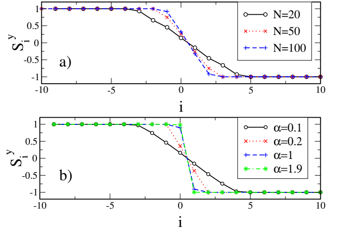
FIG. 1: (Color online) Spin values along the chain vs the spin index (only the central part of the chain has been shown) for the Hamiltonian H_y . a) for fixed \alpha = 0.1 and different N values as indicated in the legend; b) for fixed N = 20 and different \alpha values (see the legend).
