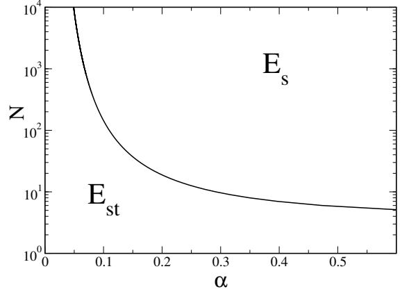
FIG. 2: Critical N_{cr} as a function of \alpha . The region above the line is where the TNT is given by E_s (one spin pair decreased) and the region below it is where the TNT has more than one spin pair decreased ( E_{st} ).
