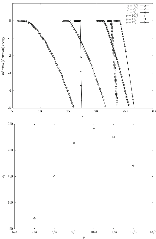
FIGURE 3. Values of the infimum (Gaussian) energy with respect to c (top) and values of c_g (bottom): from p = 7/3 to p = 12/3 they are 69.510, 150.65, 212.91, 241.01, 225.42, 170.33, respectively.
