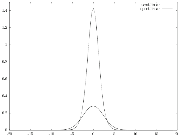
FIGURE 1. Comparison between the solution (a section of the absolute value squared) of (1.10) with \vartheta = 0 (semilinear case) and with \vartheta = 1 (quasi-linear case). The additional diffusive term present in the quasi-linear case tends to produce squeezing effects.
