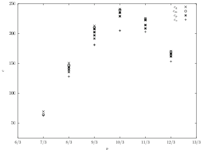
FIGURE 4. Values of c_g (Gaussian upper bound of c_{\sharp} ), c_m (values for which E(v_{c_m}(T)) < 0 ), c_p (values for which E(v_{c_p}(T)) > 0 ) and c_o (values for which the essential support of v_{c_o}(t) spreads out the computational domain). For instance, for the case p = 9/3 and c = 0.9875 \cdot c_g \approx 210.25 , we found an approximated steady state with energy E(v_c(T)) \approx -1.30 \cdot 10^{-1} (circle), whereas with c = 0.975 \cdot c_g \approx 207.59 , we found an approximated steady state with energy E(v_c(T)) \approx 6.97 \cdot 10^{-2} (star).
