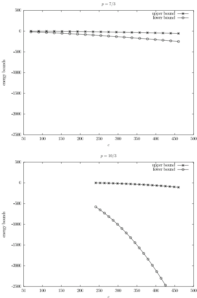
FIGURE 2. Upper and lower bounds of \mathcal{M}(c) according to the estimates obtained in Proposition 2.1 in the particular cases p = 7/3 (sharp bounds) and p = 10/3 (less sharp bounds).
